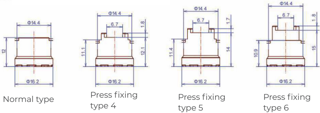
Dimensions of the main body
