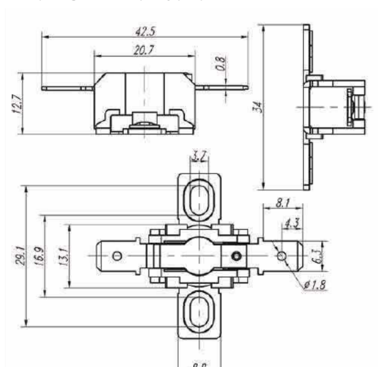
Dimensions of KSD309-A (single temp. type)
