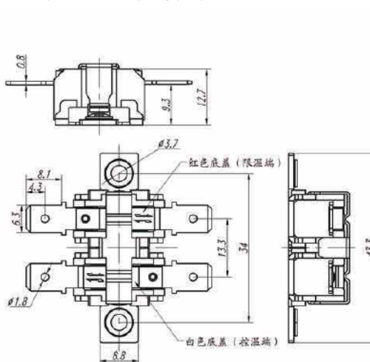
Dimensions of KSD309-A (dual temp. type)
