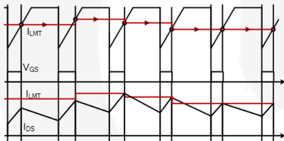
Figure 21. Current Limit Variation with Duty Cycle
