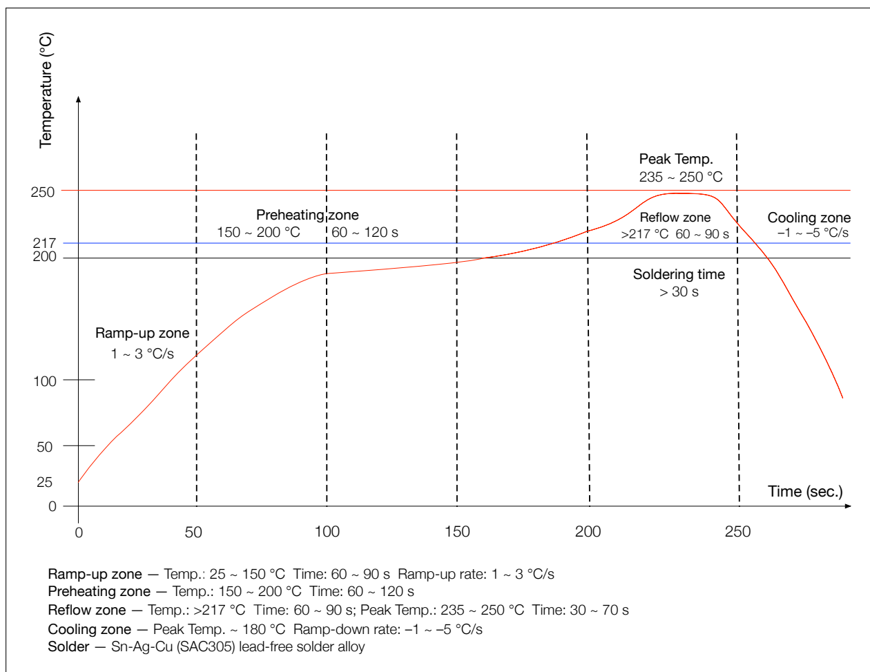
Figure 7: Reflow Profile
